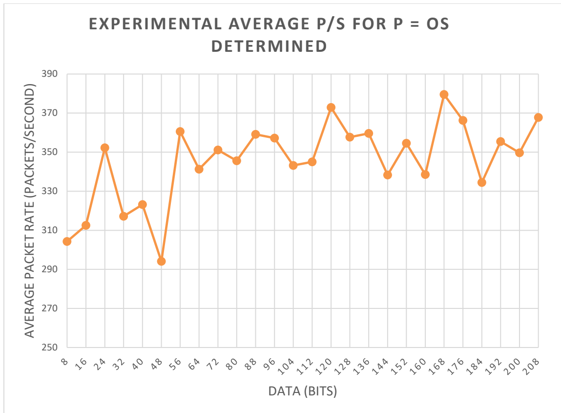
Figure 21. Average packet transfer rates for p = \text{variable } p/s
